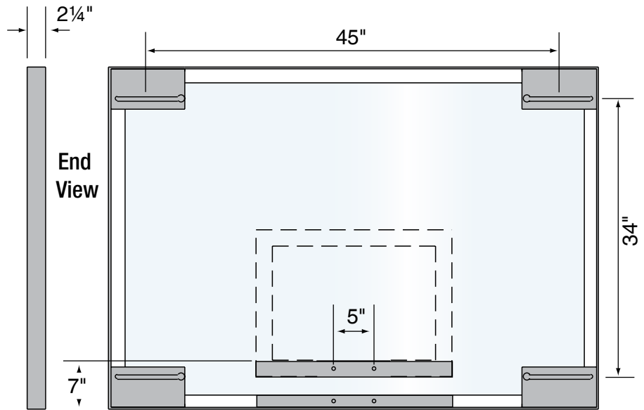
Rear View
