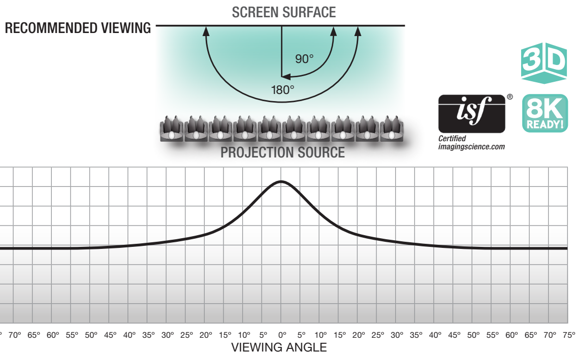
GAIN CHART TECVISION XT1800X WHITE
